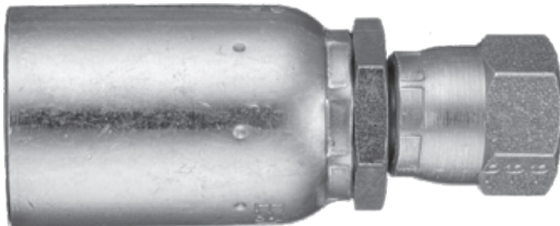
1/2" x 9/16-18 (-6) Female Swivel JIC 37° Seat
