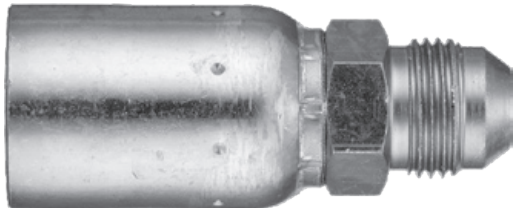
1/2" x 3/4-16 (-8) Male JIC 37° Flare
