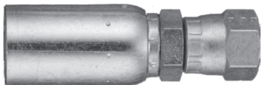
3/8" x 9/16-18 (-6) Female Swivel JIC 37° Seat
