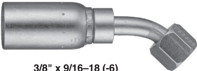
3/8" x 9/16-18 (-6) Female 45° Swivel JIC 37° Seat
