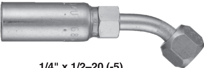
1/4" x 1/2-20 (-5) Female 45° Swivel Dual Seat
