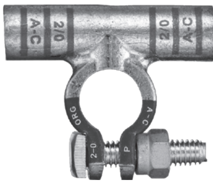
41437 Flag Post-Top Terminal 2/0 Ga. Positive
