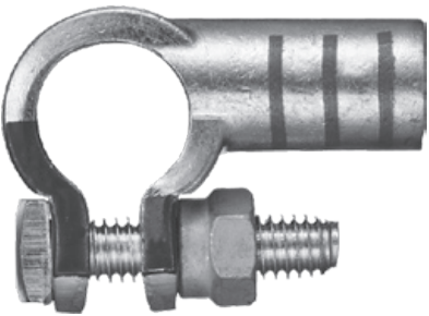
41427 Left Elbow Post-Top Terminal 1/0 Ga. Positive
