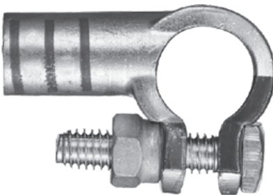
41419 Right Elbow Post-Top Terminal 1/0 Ga. Positive
