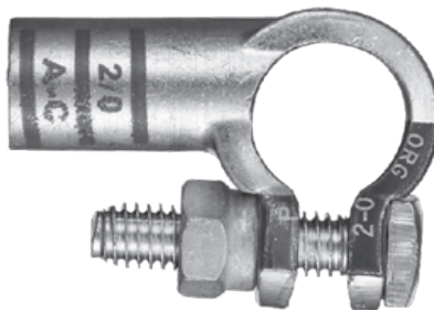
41421 Right Elbow Post-Top Terminal 2/0 Ga. Positive
