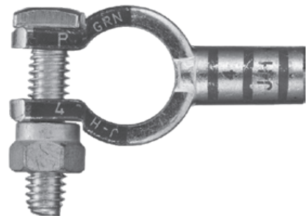
Straight Post-Top Terminal 4 Ga. Positive
