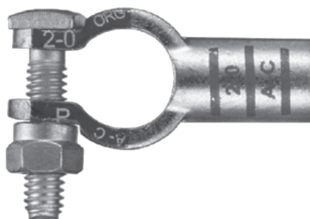
Straight Post-Top Terminal 2/0 Ga. Positive
