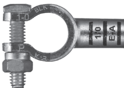
Straight Post-Top Terminal 1/0 Ga. Positive
