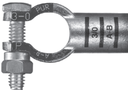
Straight Post-Top Terminal 3/0 Ga. Positive
